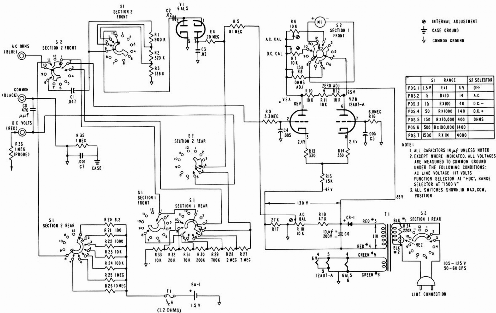
Schematic Diagram of the WV-77E
